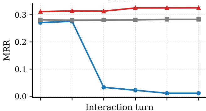
MRR
