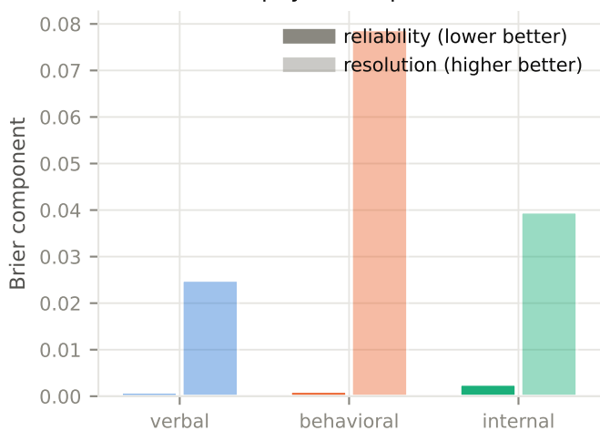
Murphy decomposition
