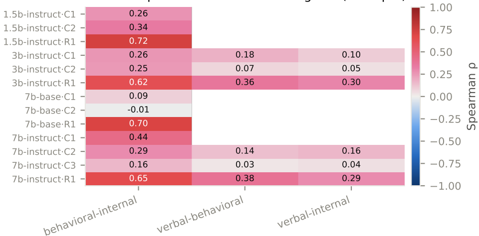
Pairwise Spearman between raw signals (test split)
