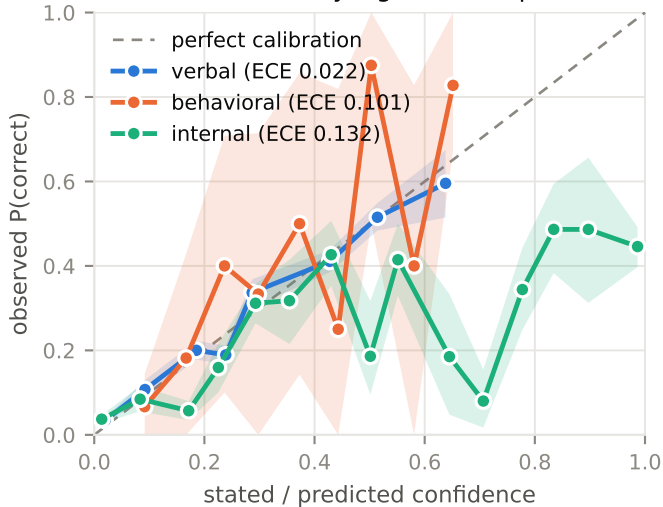
Calibration by signal (test split)
