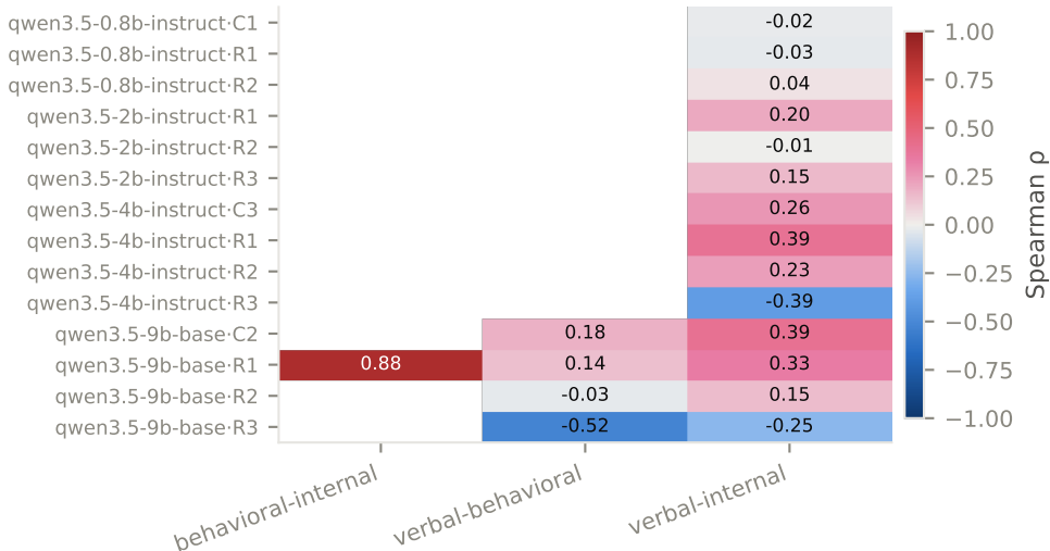
Pairwise Spearman between raw signals (test split)
