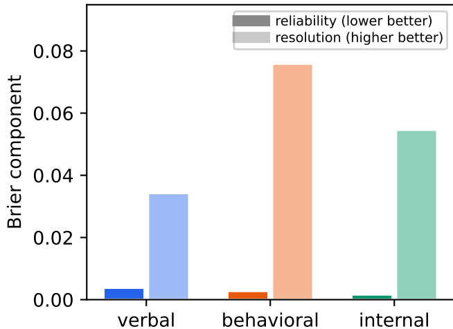
Murphy decomposition
