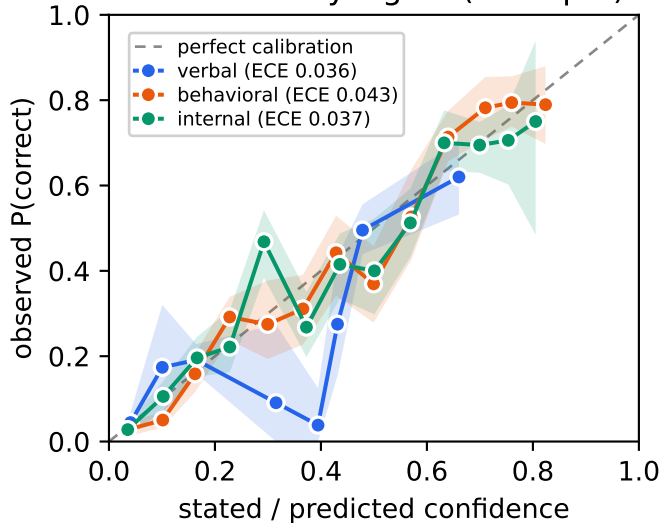
Calibration by signal (test split)
