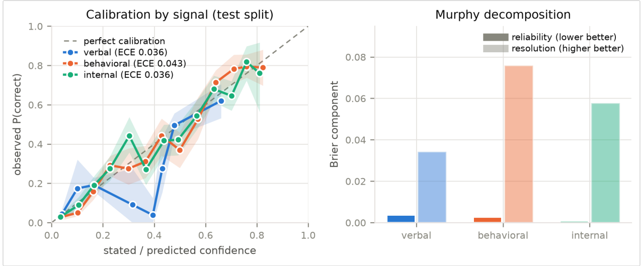
Figure 1: Signal calibration and Murphy decomposition on the test split. Left : Calibration curves hugging the diagonal; points with N < 10 pruned to remove small-sample noise. Right : Murphy decomposition of the Brier score. While all signals exhibit negligible reliability error (solid bars), behavioral consensus achieves more than double the resolution (light bars) of verbal confidence.
