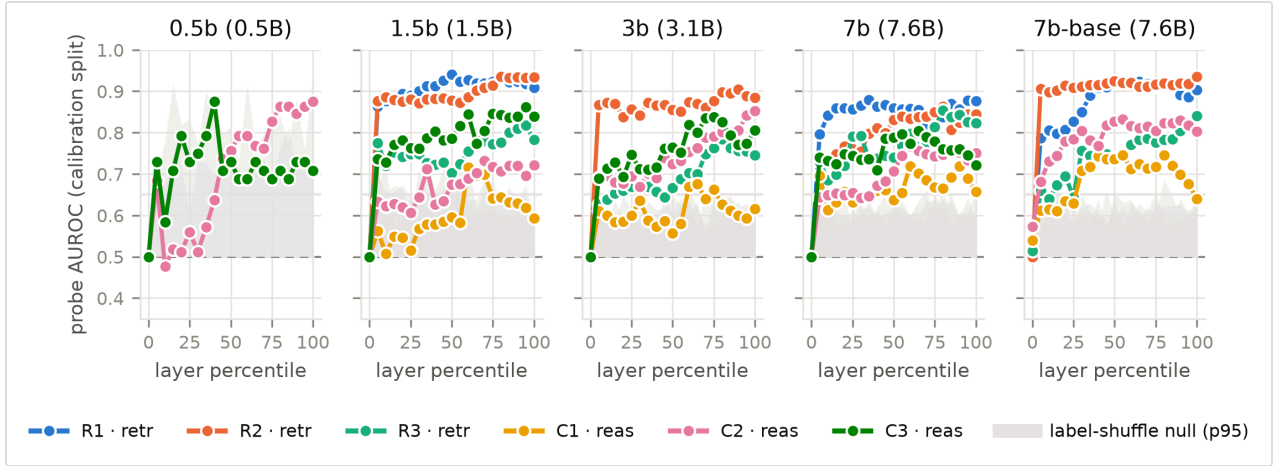
Figure 4: Continuous AUROC emergence curves across 21 layer depth percentiles. Linear probe AUROC for predicting answer correctness from prefill hidden states, faceted by model size. Retrieval tiers (solid cool lines) rise immediately above the 0.65 threshold at 5% depth. Reasoning tiers (warm lines) exhibit delayed emergence, requiring substantial depth before linear separability is achieved.
