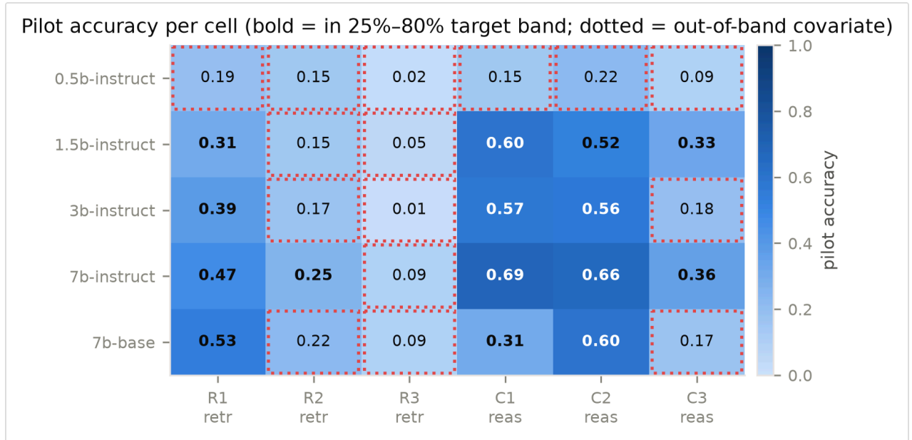
Figure 5: Complete 30-cell evaluation matrix. Pilot accuracy per (model \times tier) cell. All 30 cells were committed across 4.778 GPU-hours on an NVIDIA RTX PRO 6000 Blackwell Server Edition; dotted outlines indicate cells outside the 25%–80% accuracy band controlled via in_band covariates.
