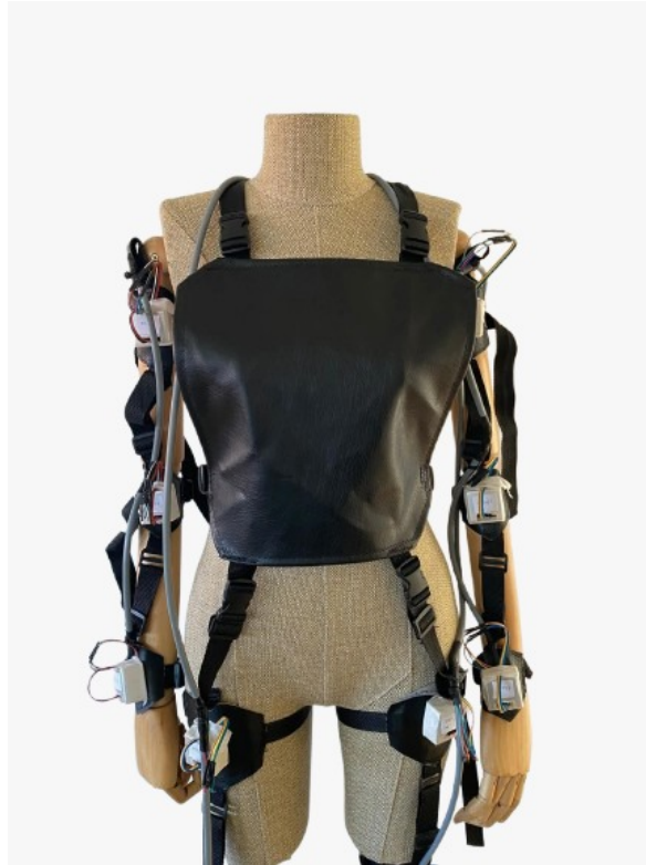
Figure 4.3: Assembled MotionSuit with 14-Sensor Layout.
