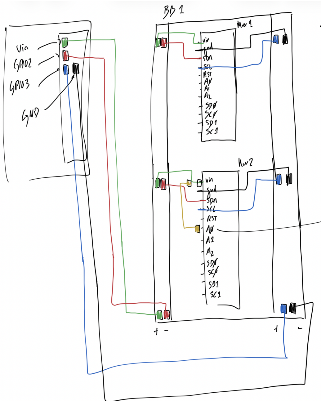
Figure 4.1: I2C Multiplexer and Sensor Wiring Schematic.
