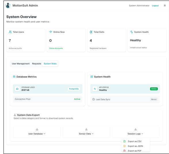
(b) Final System Stats Interface.
