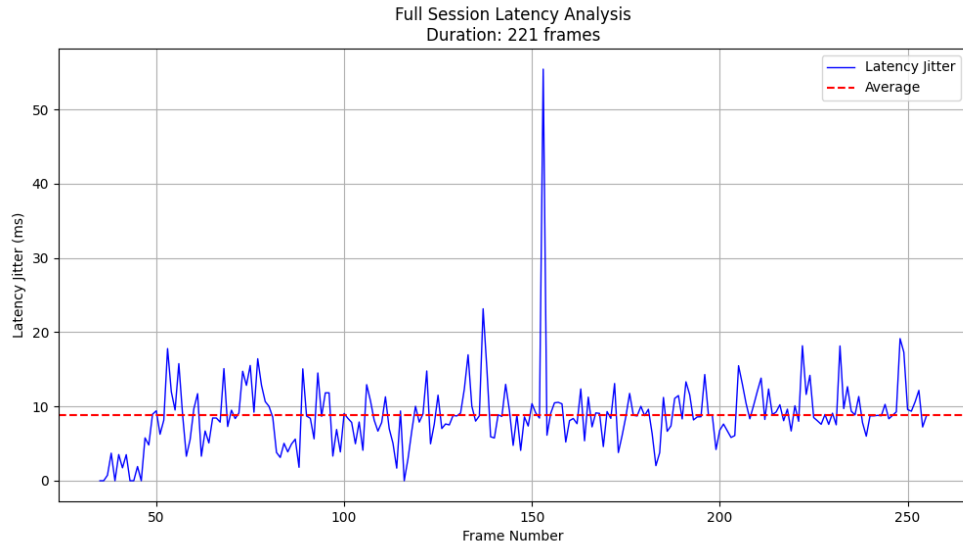
(b) Real Sensor Latency ( \approx 9.5 ms).
