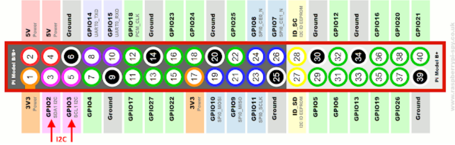
Figure 4.2: Raspberry Pi 40 Pin Header.
