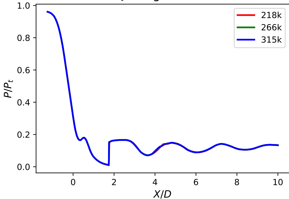
P/P_t along centerline
