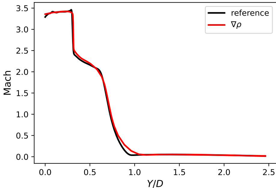
Mach at X/D = 1.54
