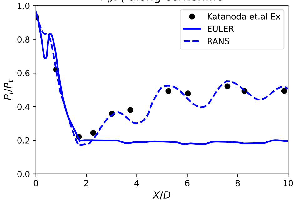
P_i/P_t along centerline
