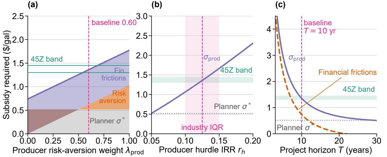
Figure 2: Comparative statics of \sigma_{\text{prod}}
