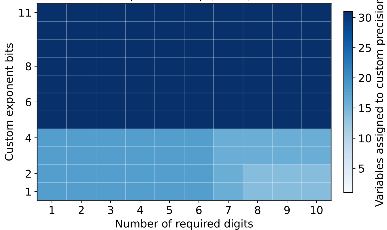
Exponent sweep ( t = 52 )
