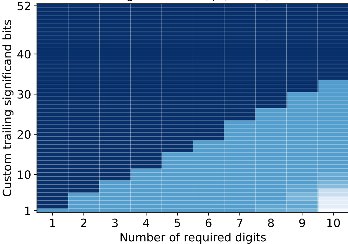
Significand sweep ( e = 11 )
