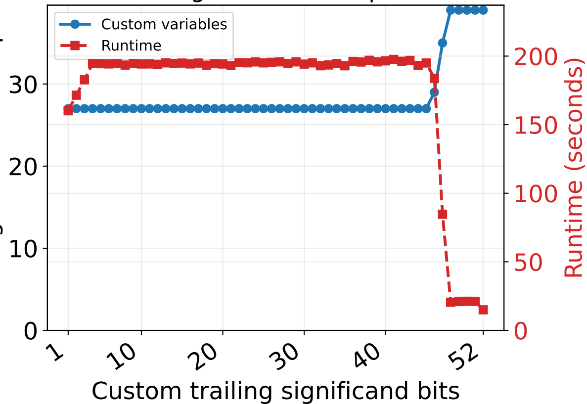
Custom significand sweep, e = 11
