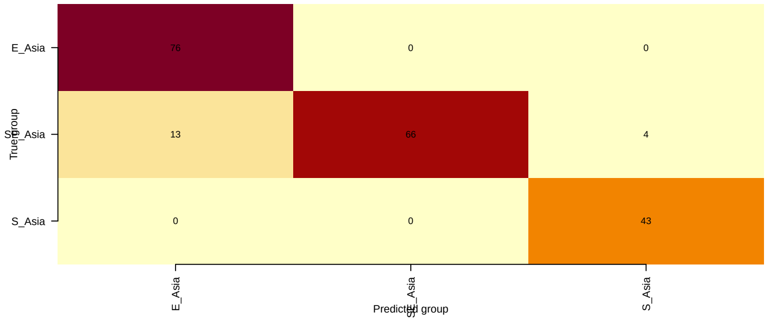
P3_subregion_within_asia LOO confusion matrix
