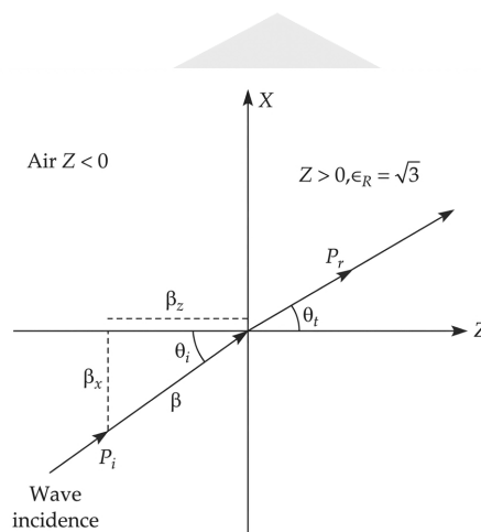
Fig. Solution Q2.14.1
