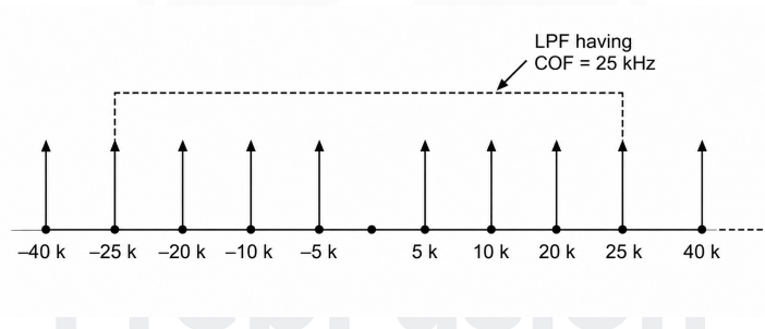
Fig. Solution Q4.20.2
