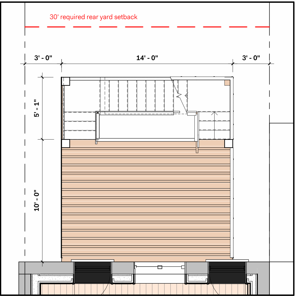
3 DECK OPTION 2 - 001 ENLARGED PLAN 1/4" = 1'-0"
