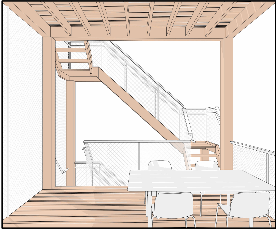
6 DECK OPTION 2 - PERSPECTIVE
