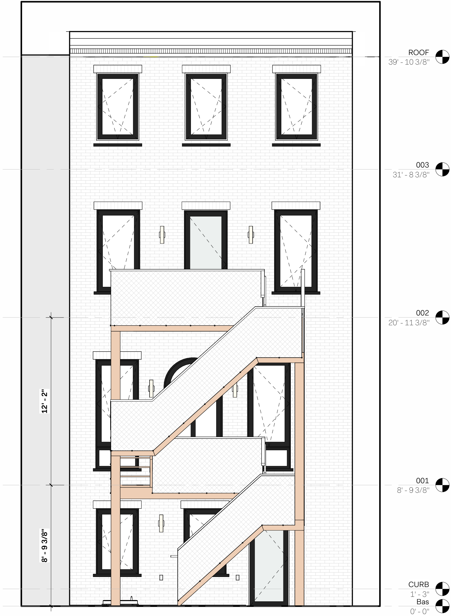
4 DECK OPTION 2 - ELEVATION 1/4" = 1'-0"
