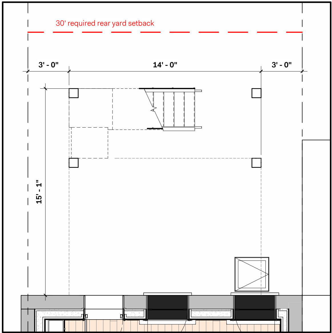
2 DECK OPTION 2 - BAS ENLARGED PLAN 1/4" = 1'-0"
