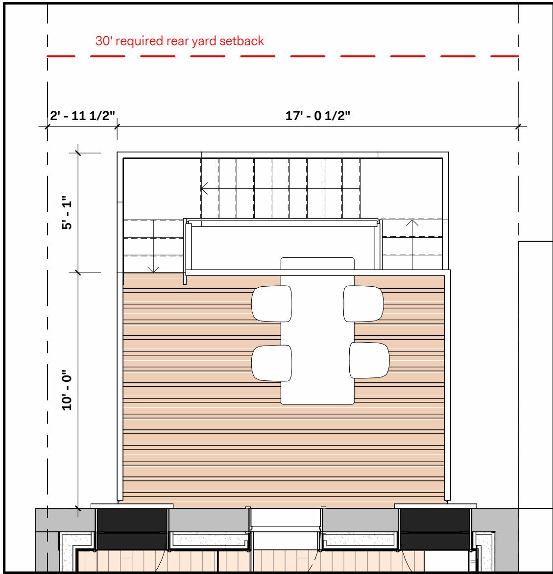
5 DECK OPTION 2 - 002 ENLARGED PLAN 1/4" = 1'-0"
