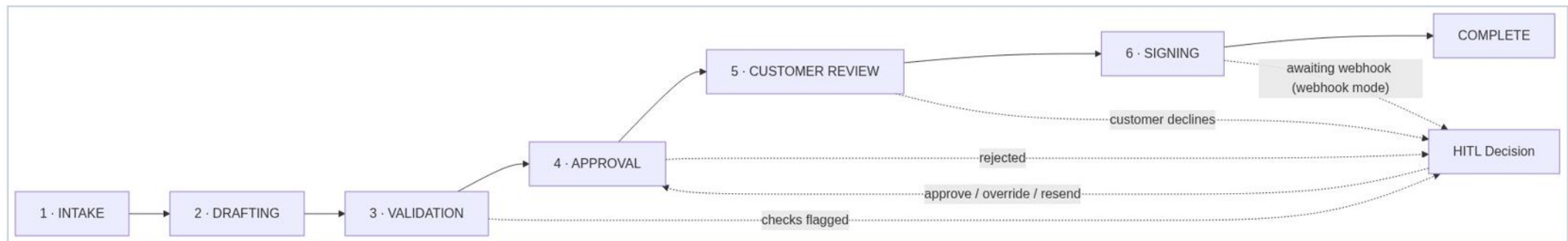
Fig 2 — Lifecycle: the resumable six-stage state machine
