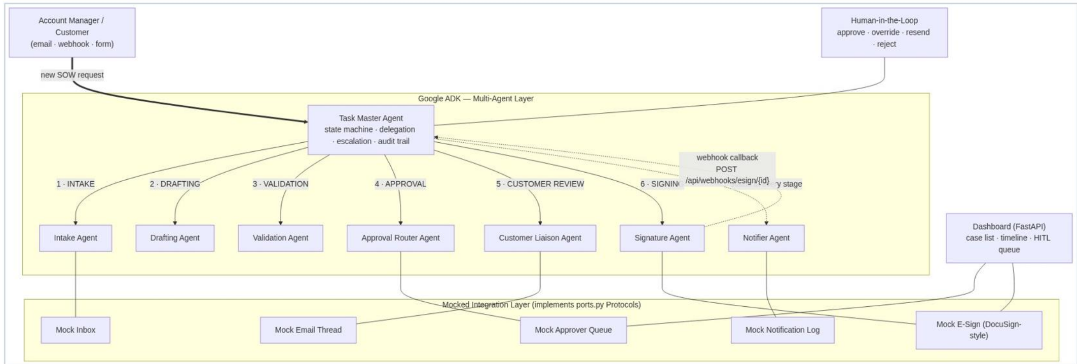
Fig 1 — Agent graph: orchestrator, supporting agents, mock integration layer, HITL
