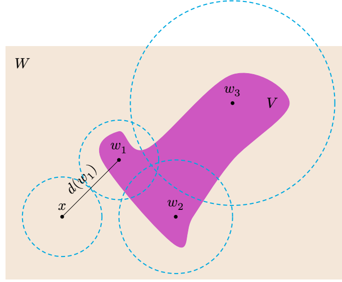
Figure 3.1.: If W is compact and V \subseteq W is closed, then for every x \in W \setminus V one can find \varepsilon such that B_\varepsilon(x) \subseteq W \setminus V .
