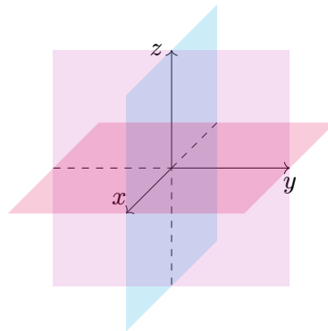
Figure 1: The union of the three coordinate planes.
