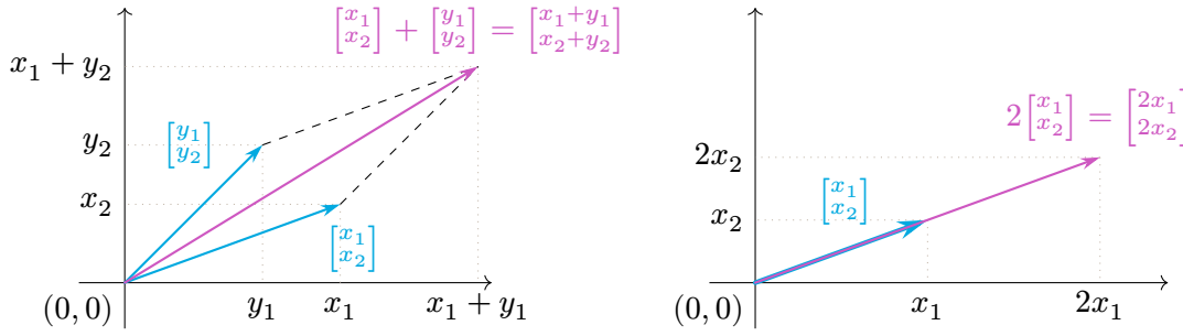
Figure 2.2.: Addition and scalar multiplication (by 2) \mathbf{R}^2 .
