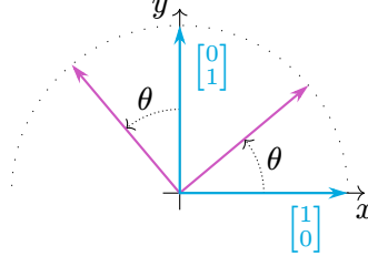
Figure 3.4.: Rotation (in purple) of the standard basis vectors (in blue) by an angle \theta .
