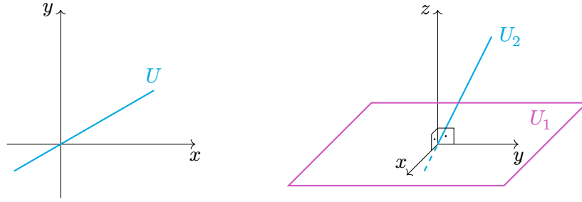
Figure 2.3.: On the left: a line containing the origin in \mathbf{R}^2 . On the right: a plane and a line containing the origin in \mathbf{R}^3 .
