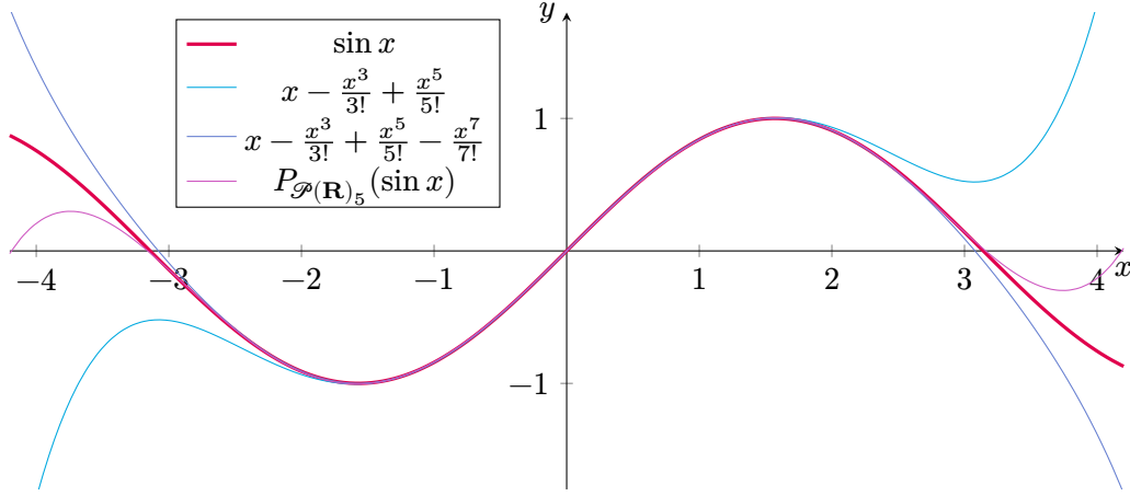
Figure 4.14.: Three polynomial approximations of the sine function. By the Taylor polynomials of degree 5 and 7, and a better one by the projection on \mathcal{P}(\mathbf{R})_5 .
