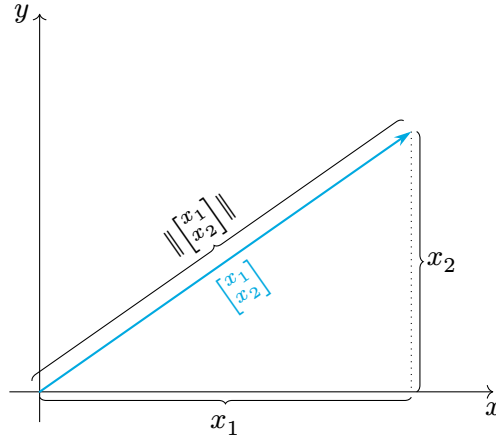
Figure 4.1.: The norm of the vector \begin{bmatrix} x_1 \\ x_2 \end{bmatrix} \in \mathbf{R}^2 is \left\| \begin{bmatrix} x_1 \\ x_2 \end{bmatrix} \right\| = \sqrt{x_1^2 + x_2^2} .
