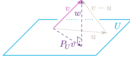
Figure 4.13.: The orthogonal projection of v onto U , with “error” \|w\| = \|v - P_U(v)\| and a worst approximation u with error \|v - u\| > \|v - P_U(v)\| .
