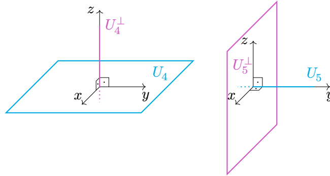
Figure 4.11.: Orthogonal complements in \mathbf{R}^3 .
