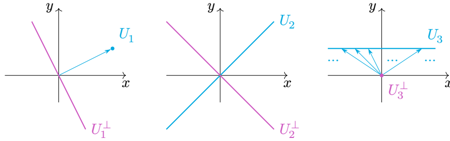
Figure 4.10.: Orthogonal complements in \mathbf{R}^2 .
