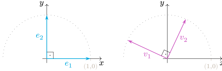
Figure 4.9.: Two orthonormal bases of \mathbf{R}^2 . Any orthonormal basis of \mathbf{R}^2 can be obtained by a rotation from (e_1, e_2) or from (e_2, e_1) .
