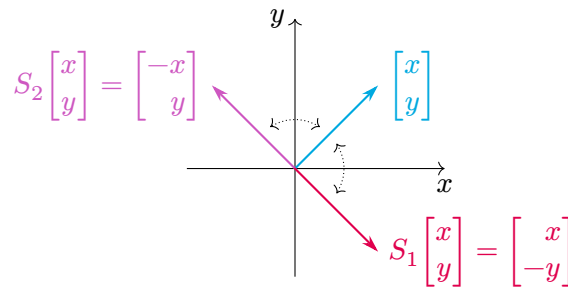
Figure 3.7.: Mirror symmetries with respect to the x -axis ( S_1 ) and the y -axis ( S_2 ).
