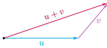
Figure 4.6.: The shortest path between the black dot and the greydot is given by the vector u + v . This figure explains the name “triangle inequality”.
