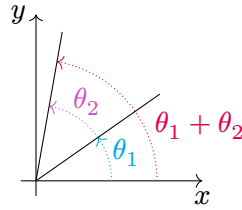
Figure 3.6.: Angles addition.
