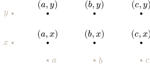
Figure 1.2.: A graphic representation of the product \{a, b, c\} \times \{x, y\} .
