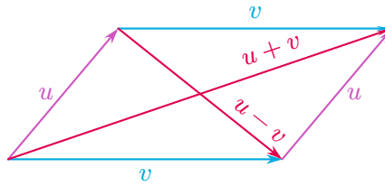
Figure 4.7.: A parallelogram and its two diagonals, explaining the name of the theorem. The identity means that in a parallelogram the sum of the square of the diagonal lengths is equal to the sum of the square of the side lengths.
