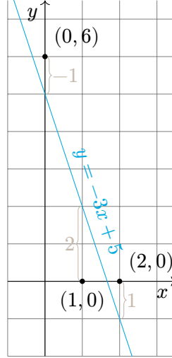
Figure 4.15.: Best-fit line for the three black dots. The error is \sqrt{6} .
