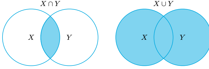
Figure 1.1.: Intersection and union of two sets. The white parts in the diagram contains no elements.
