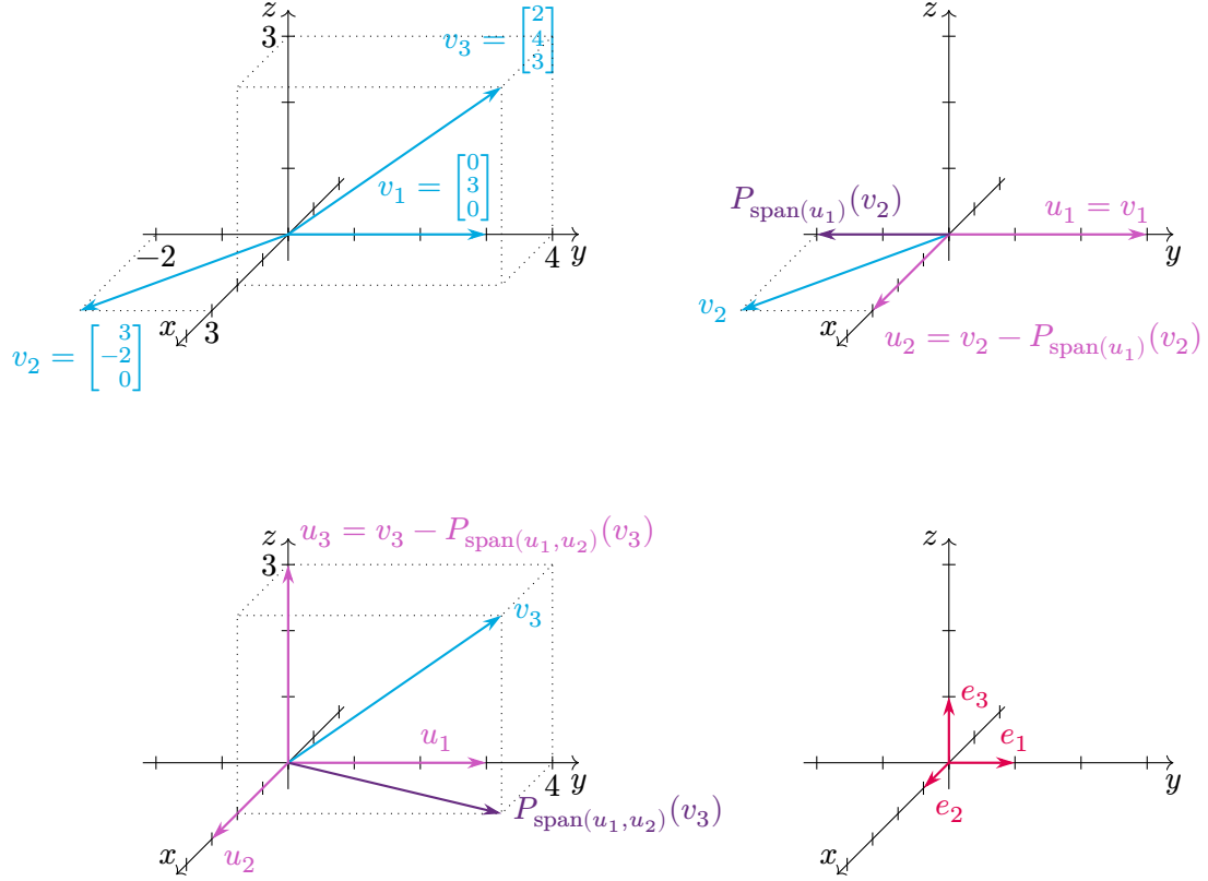
Figure 4.12.: The Gram–Schmidt procedure applied to the linearly independent list (v_1 = \begin{bmatrix} 0 \\ 3 \\ 0 \end{bmatrix}, v_2 = \begin{bmatrix} 3 \\ -2 \\ 0 \end{bmatrix}, v_3 = \begin{bmatrix} 2 \\ 4 \\ 3 \end{bmatrix}) (top left). We first put u_1 = v_1 and compute u_2 = v_2 - P_{\text{span}(u_1)}(v_2) (top right). We then compute u_3 = v_3 - P_{\text{span}(u_1, u_2)}(v_3) (bottom left). Finally we normalise the vectors to obtain the orthonormal list (\begin{bmatrix} 1 \\ 0 \\ 0 \end{bmatrix}, \begin{bmatrix} 0 \\ 1 \\ 0 \end{bmatrix}, \begin{bmatrix} 0 \\ 0 \\ 1 \end{bmatrix}) (bottom right).
