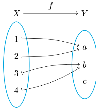
Figure 1.3.: The function f: \{1, 2, 3, 4\} \rightarrow \{a, b, c\} defined by f(1) = f(2) = a and f(3) = f(4) = b . No element of \{1, 2, 3, 4\} is sent onto c .
