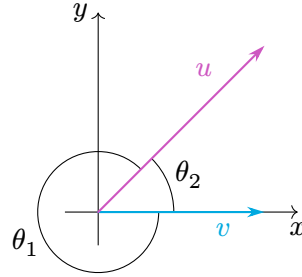
Figure 4.5.: The angle between u and v is the minimum between \theta_1 and \theta_2 = 2\pi - \theta_1 .
