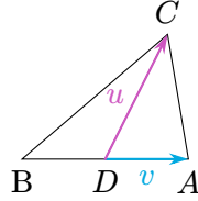
Figure 4.8.: A triangle ABC , where D is the midpoint of AB .
