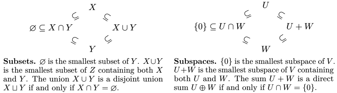
Figure 2.6.: Comparisons between subsets X and Y of a set Z and subspaces U and W of a vector space V . The intersection X \cap Y ( U \cap W ) is the biggest subset (subspace), of Z (of V ), contained both in X and Y ( U and W ).
