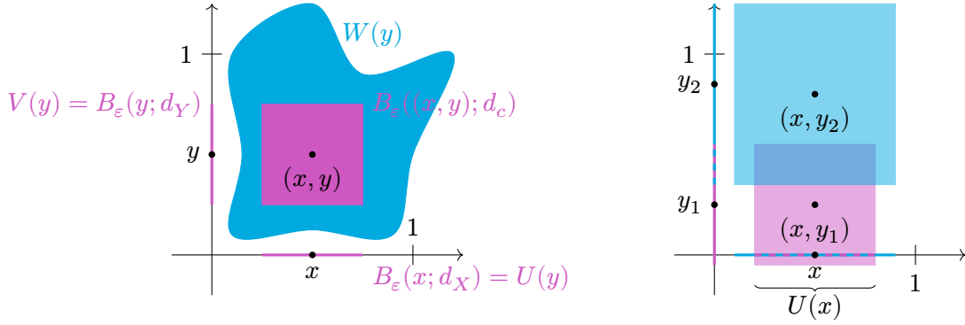
Figure 3.2.: The construction of the (good) subset U(x) \subseteq [0, 1] . One see that (the band) U(x) \times [0, 1] is contained in B_\varepsilon((x, y_1); d_c) \cup B_\varepsilon((x, y_2); d_c) (the union of the two squares), and hence in W(y_1) \cup W(y_2) .
