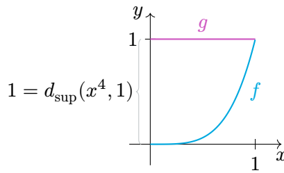
Figure 1.5.: Graphs of the polynomial functions f(x) = x^4 and g(x) = 1 . The d_{\sup} distance between the functions is the supremum of the vertical distance between their graphs.
