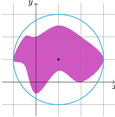
Figure 1.9.: A subset of \mathbf{R}^2 of diameter 2.
