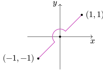
Figure 2.5.: A path from (-1, -1) to (1, 1) that avoids 0.
