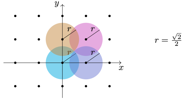
Figure 3.3.: Every point in \mathbf{R}^2 is at distance at most \frac{\sqrt{2}}{2} of a point with integer coordinates (represented by black dots).
