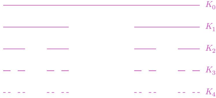
Figure 5.1.: Construction of the Cantor Set.
