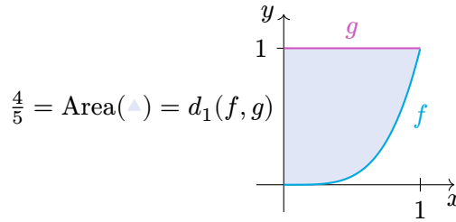
Figure 1.6.: Graphs of the polynomial functions f(x) = x^4 and g(x) = 1 . The d_1 distance between the functions is the area of the surface between their graphs.
