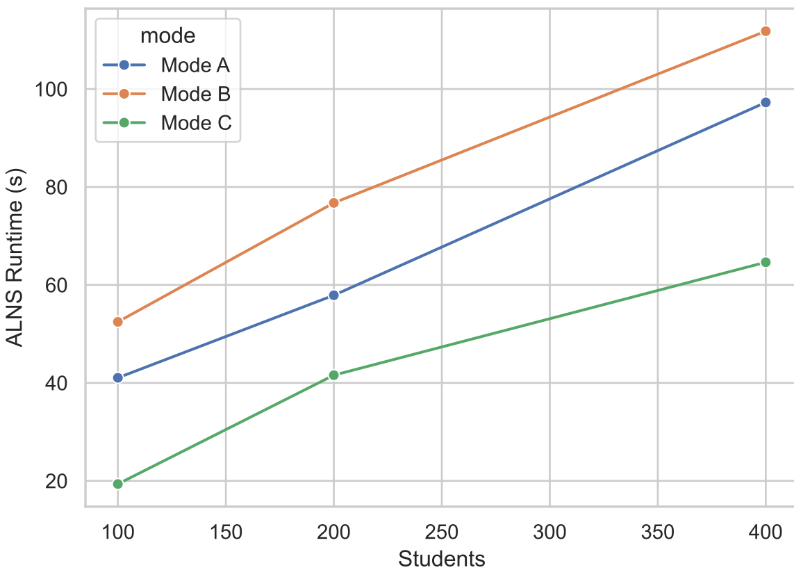
Runtime vs Problem Size
