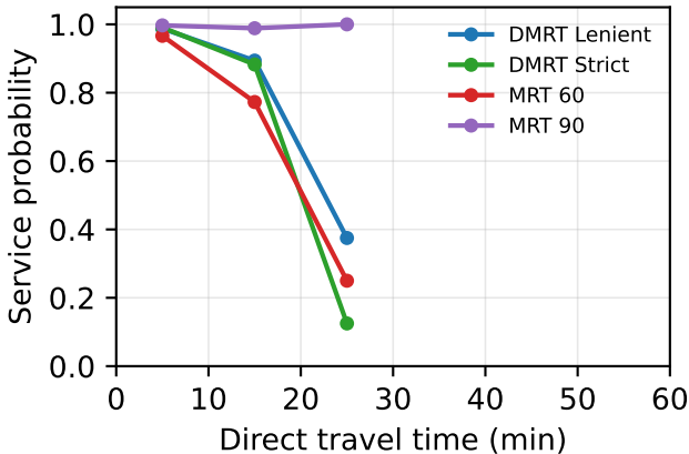
Service Probability vs Direct Time ( |S|=200 )
