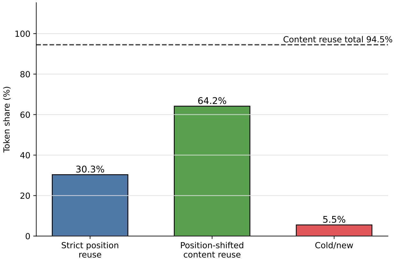
Previous-request context reuse breakdown
