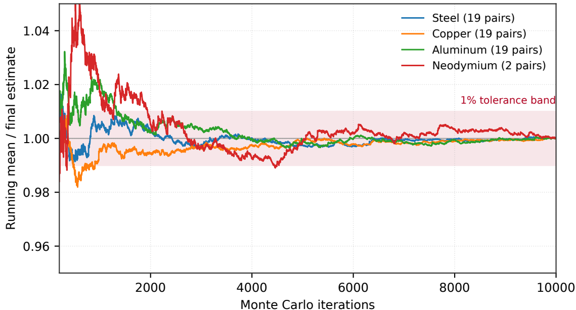
Monte Carlo convergence (representative materials, seed 24601)
