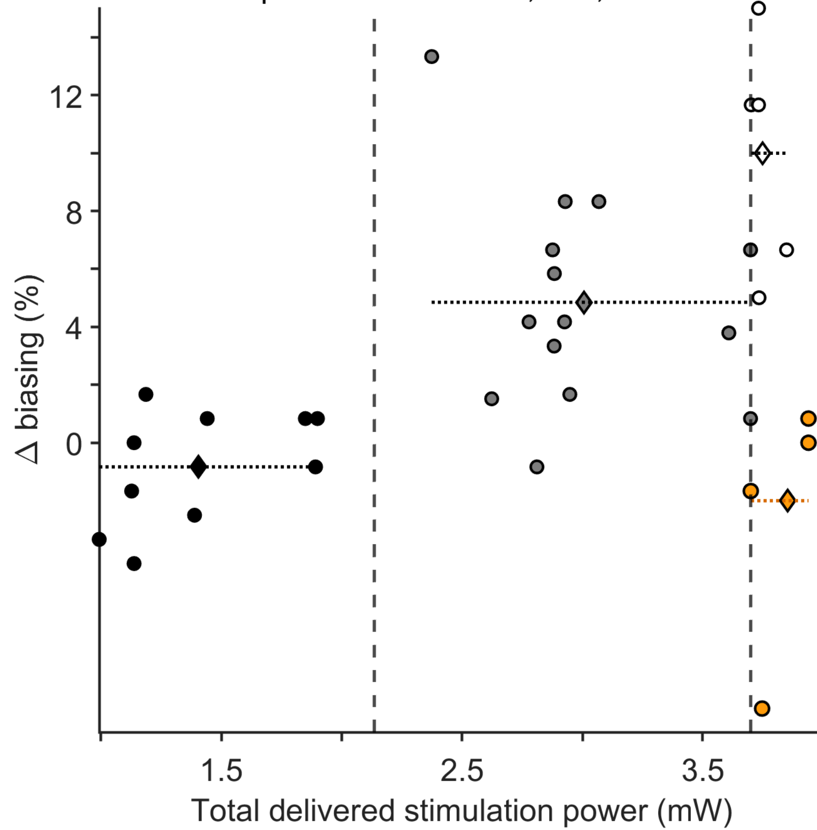
Ordered power-effect bands, k=3, score=0.419
