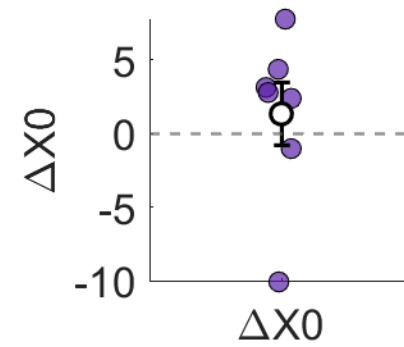
Power cluster 2 individual Weibull parameters, Columns 0^\circ/90^\circ ( n_{\text{expt}}=7 ) | signed-BX0 individual parameters
