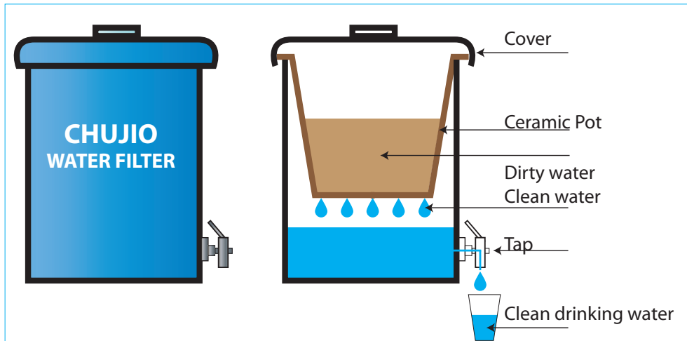
Chujio water filter.
