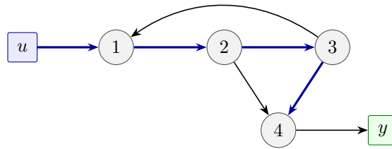
Figure 4.1: The pattern graph of Example 2.4: same picture as Fig. 2.1, numbers erased. It is the running example for this section. The stem u \rightarrow 1 \rightarrow 2 \rightarrow 3 \rightarrow 4 (bold) covers all state nodes.
