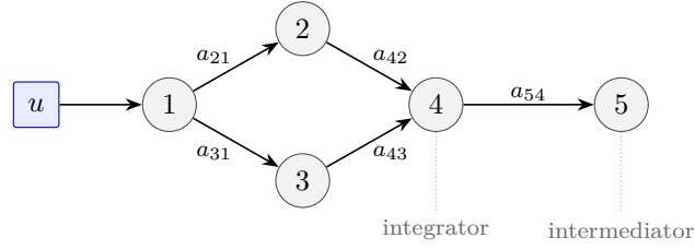
Figure 4.4: One edge 4 \rightarrow 5 of weight a_{54} appended to the diamond of Example 6.2 . Node 4 collects two in-edges and is an integrator; node 5 has a single in-neighbor, but every stem to it runs through node 4, so it is an intermediary ( Definition 4.30 ) and inherits the multi-term, [\mathcal{C}_F]_{5,4} = a_{54}(a_{21}a_{42} + a_{31}a_{43}) .
