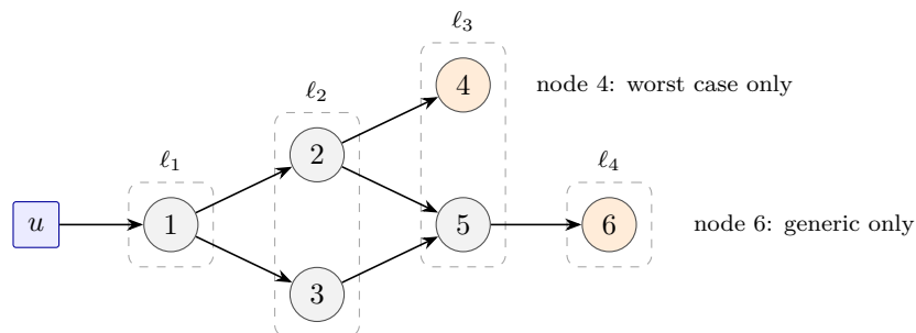
Figure 8.3: The pattern of Remark 8.3 : driver 1, state edges 1 \rightarrow 2 , 1 \rightarrow 3 , 2 \rightarrow 4 , 2 \rightarrow 5 , 3 \rightarrow 5 , 5 \rightarrow 6 , and the distance layers \ell_1 = \{1\} , \ell_2 = \{2, 3\} , \ell_3 = \{4, 5\} , \ell_4 = \{6\} of this input-connected HDAG. The two edges into node 5 carry the weight products whose sum a_{21}a_{52} + a_{31}a_{53} is the entry [\mathcal{C}_F]_{5,3} , and every other multi-term of the pattern is a multiple of it: generically \dim \mathcal{C}_\Lambda = 4 , and where that sum vanishes \dim \mathcal{C}_\Gamma = 3 . Which intersection each shaded node survives is what separates the two readings of the FSSCS. Node 4 lies in the intersection over the worst-case realizations, \text{span}\{e_1, e_4\} , and in the controllable subspace of no generic realization, so it is neither an FSC nor an FSSC node; node 6 lies in the intersection over the generic realizations, \mathcal{C}_\Lambda^F = \text{span}\{e_1, e_6\} , and not in \mathcal{C}_\Gamma^F = \text{span}\{e_1\} , the intersection over the whole family taken by Definition 8.2 .
