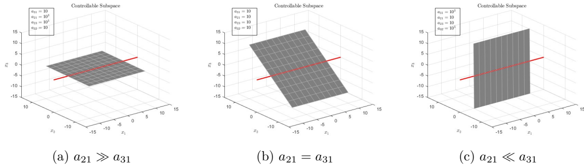
Figure 8.2: Three worst-case realizations of Example 8.1, all with a_{21}^2 a_{32} = a_{23} a_{31}^2 (figures from the author's dissertation [15]). The controllable plane \text{span}\{e_1, a_{21}e_2 + a_{31}e_3\} rotates about the x_1 -axis (red line): (a) a_{21} = 10^3 , a_{23} = 10^5 , a_{31} = a_{32} = 10 — almost the x_1x_2 -plane; (b) all weights 10 — the diagonal position; (c) a_{31} = 10^3 , a_{32} = 10^5 , a_{21} = a_{23} = 10 — almost the x_1x_3 -plane. The axis common to every position is the fixed subspace.
