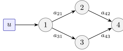
Figure 6.1: The diamond of Example 6.2 : two equal-length paths to node 4 make its column a multi-term (it can become zero), and one input for the twins 2, 3 caps the generic dimension at three.
