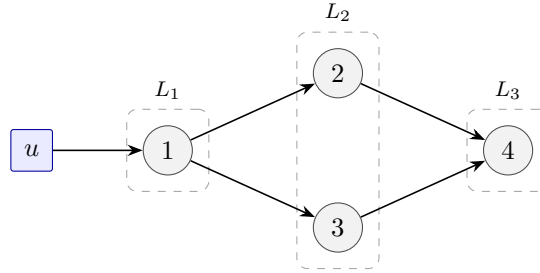
Figure 4.2: The diamond of Example 4.22 arranged into distance layers L_1 = \{1\} , L_2 = \{2, 3\} , L_3 = \{4\} : every walk from the input to a node has a single length, so the pattern is a hierarchical DAG. The four-node network of Fig. 4.1, whose node 4 sits at two different distances, is not.
