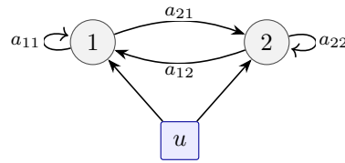
Figure 3.2: Example 3.12 : one graph, two weight assignments, opposite controllability verdicts — the graph alone cannot decide, but it can say when the numbers matter, which is the subject of Part II.
