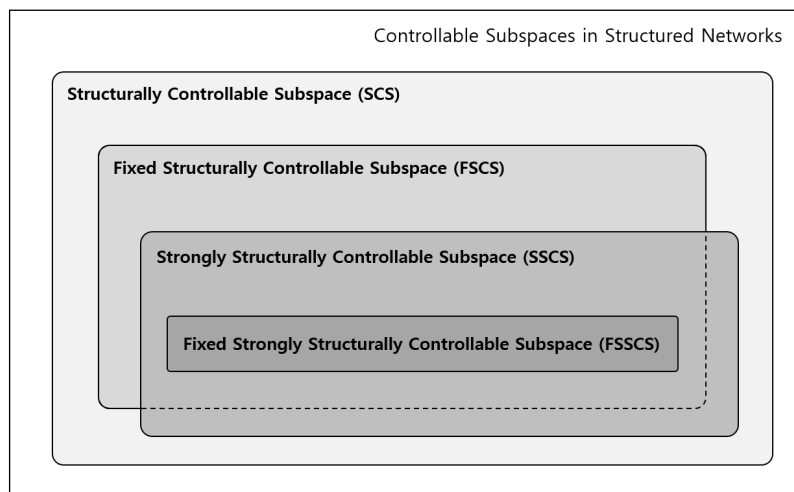
Figure 6.2: The four controllable subspaces of a structured network and their inclusions (figure from the author’s dissertation [14] ; the four-subspace framework was introduced in [10] ). This chapter concerned the outer pair SCS/SSCS; Chapter 8 enters the fixed pair.
