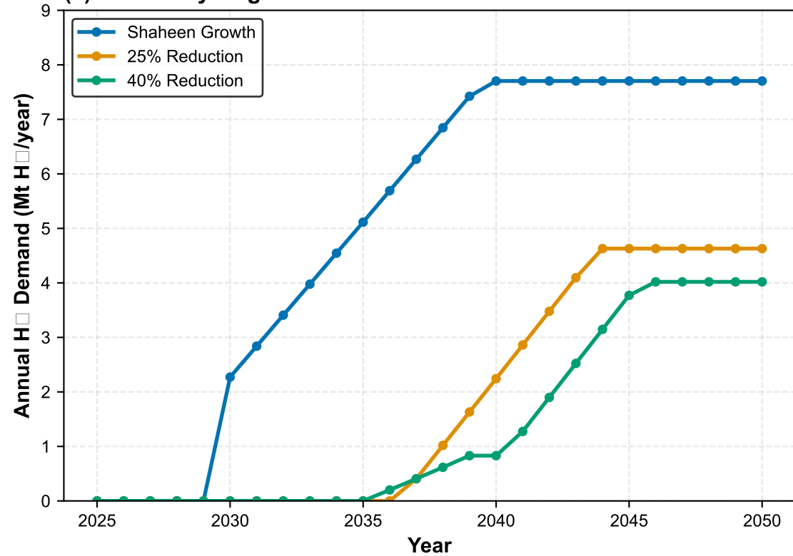
(a) Annual Hydrogen Demand
