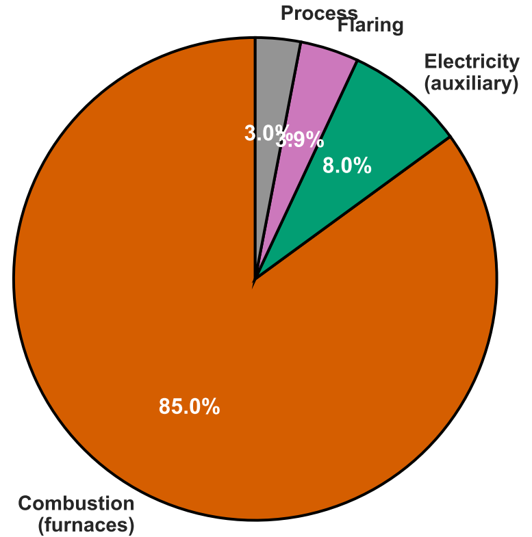
(b) Emissions by Source Combustion dominates (85%)
