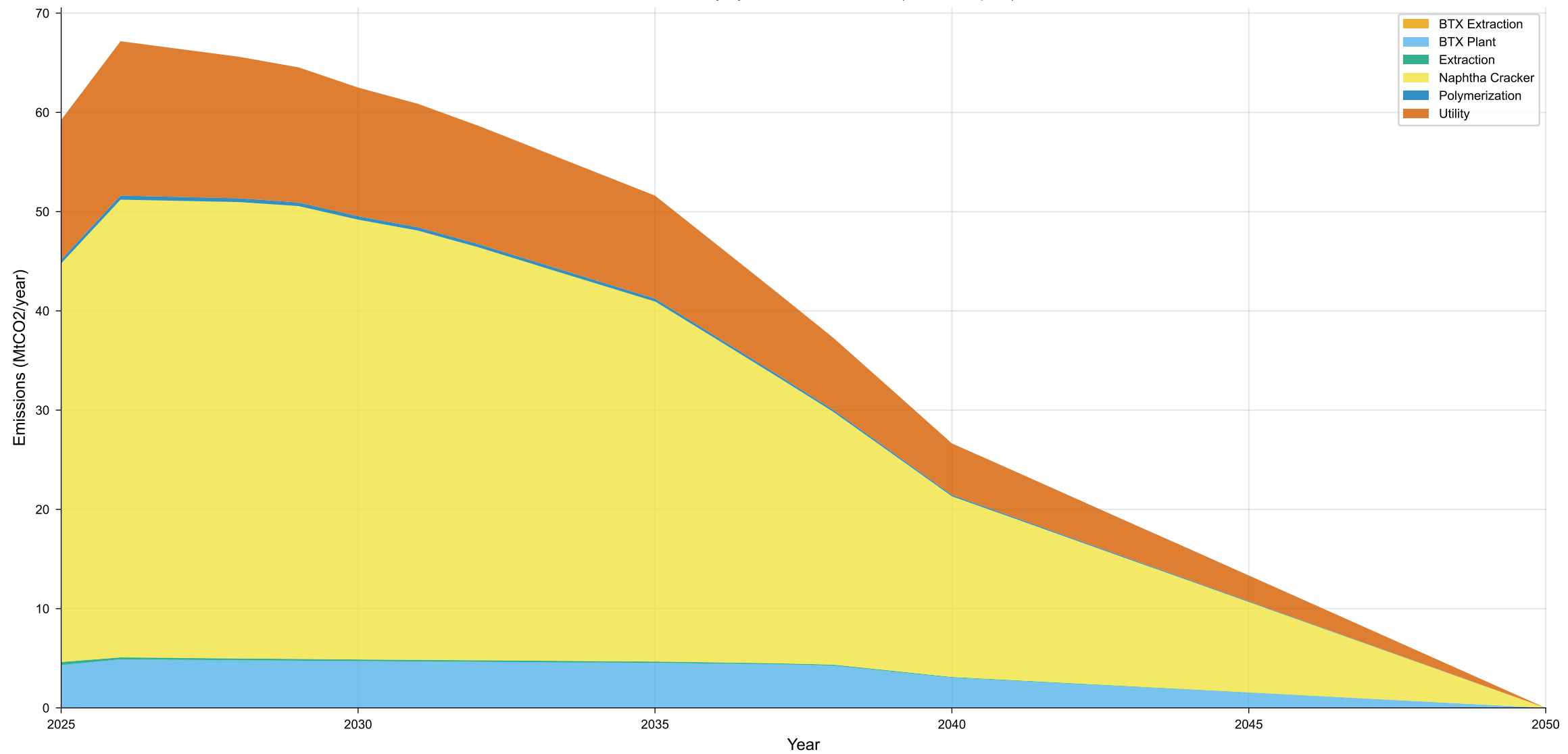
Emission Pathway by Process - NCC-Elec (Flat + Coupled)
