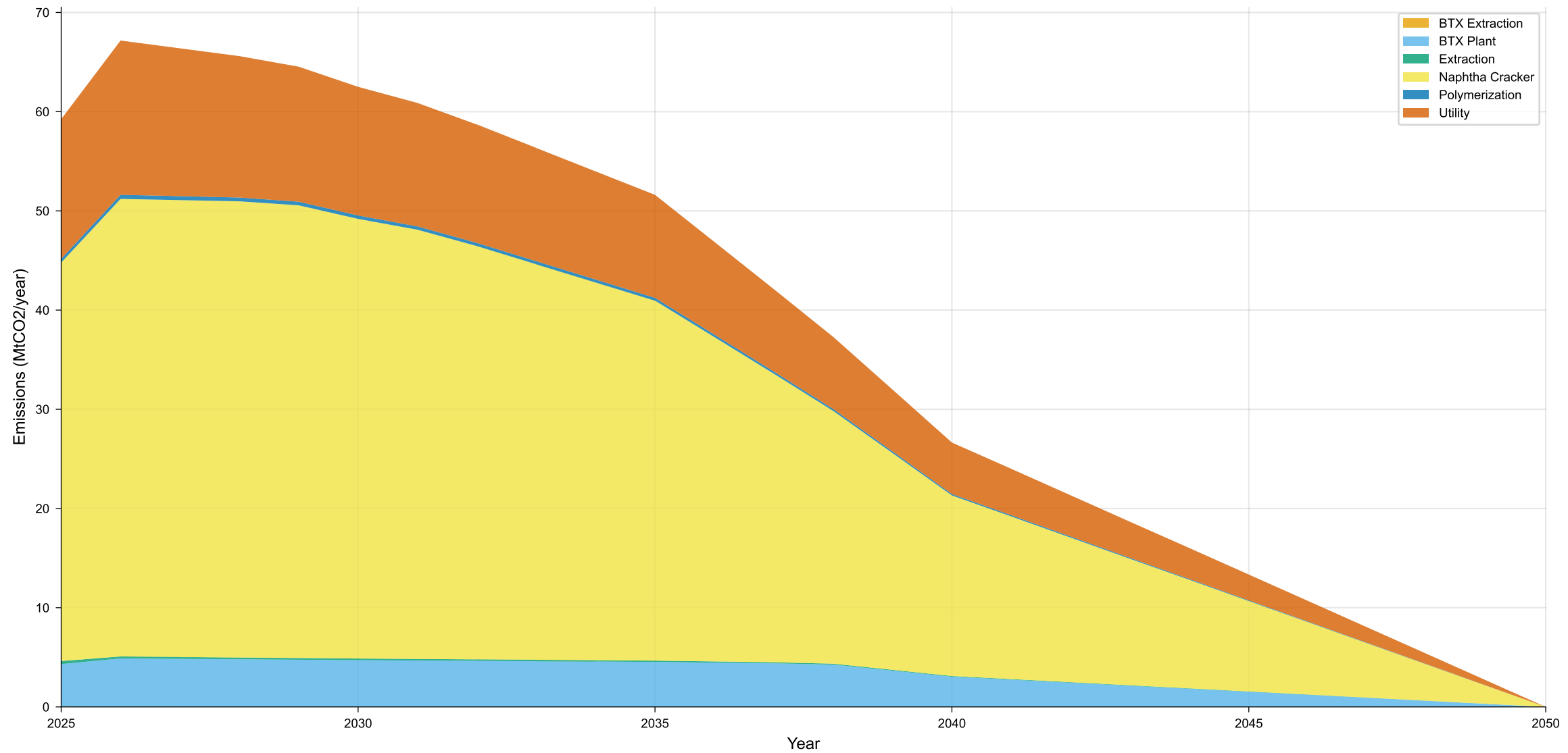
Emission Pathway by Process - NCC-Elec (Rising + Decoupled)
