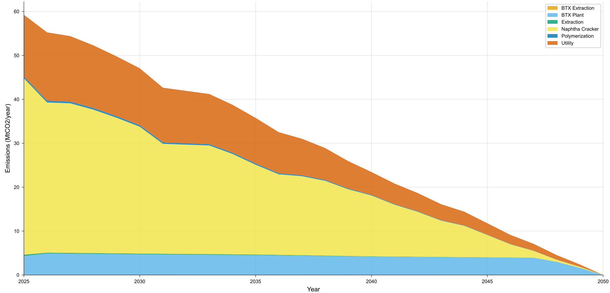
Emission Pathway by Process - NCC-H2 (Rising + Decoupled)
