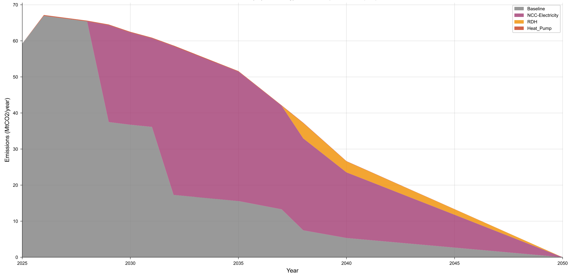
Emission Pathway by Technology - NCC-Elec (Flat + Decoupled)
