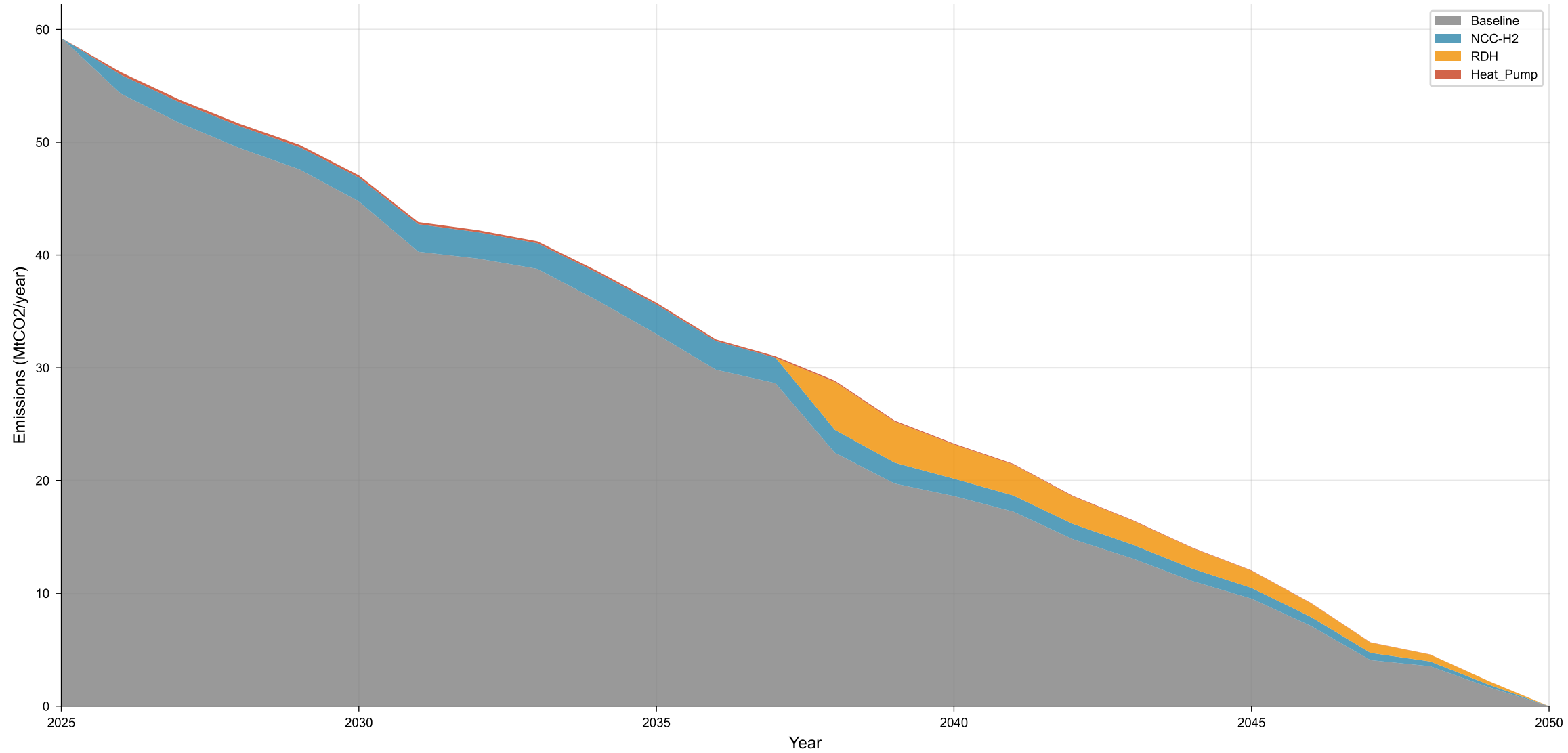
Emission Pathway by Technology - NCC-H2 (Flat + Decoupled)
