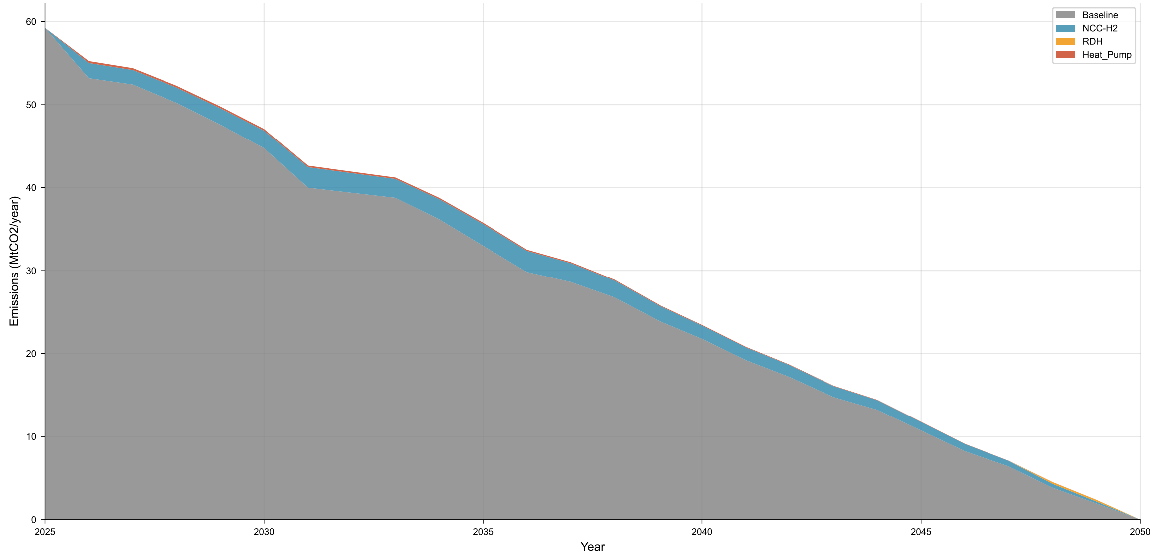
Emission Pathway by Technology - NCC-H2 (Rising + Decoupled)
