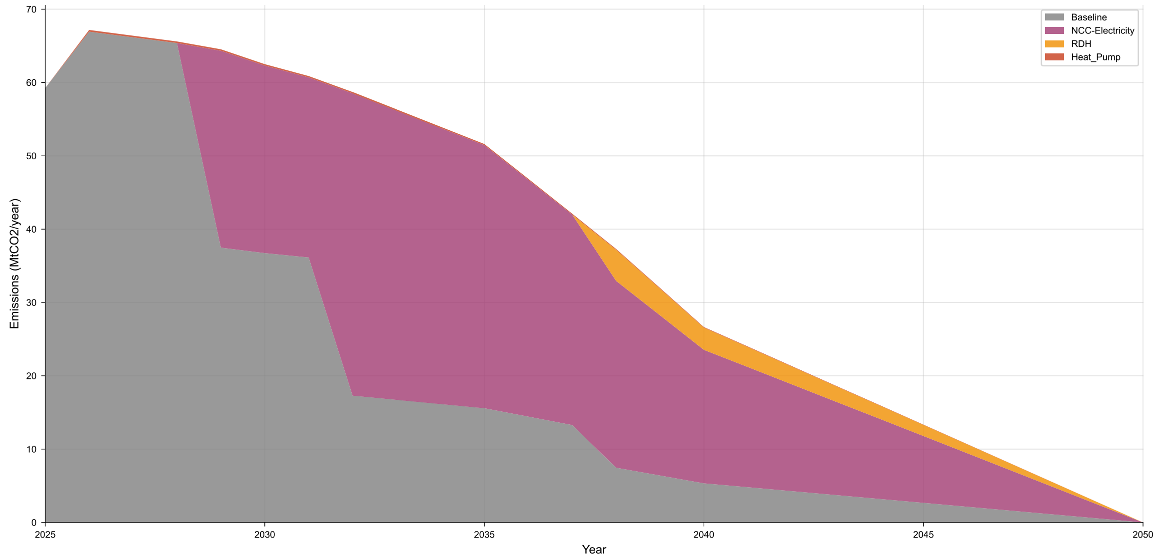
Emission Pathway by Technology - NCC-Elec (Rising + Coupled)
