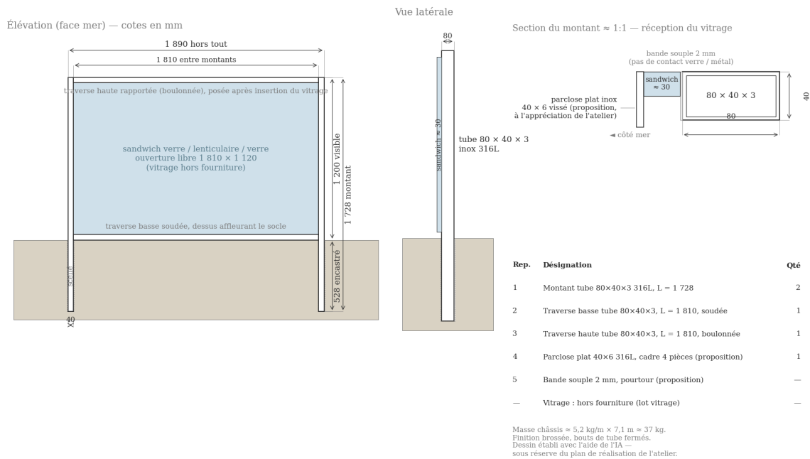
Fig. 3 — Frame v02: elevation, side view, upright section, parts list (LV-VL-CH-02; drawing labelled in French).
