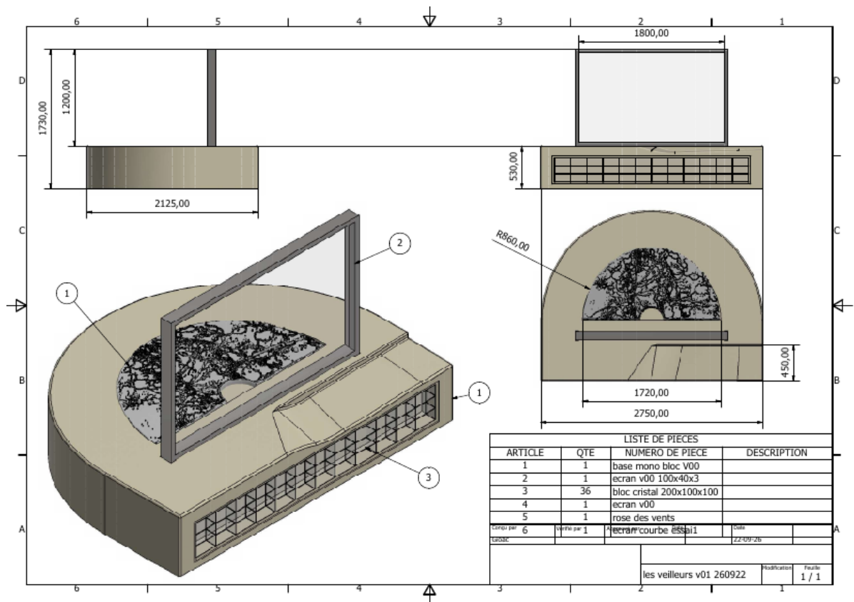
Fig. 2 — Position of the screen on the base.
