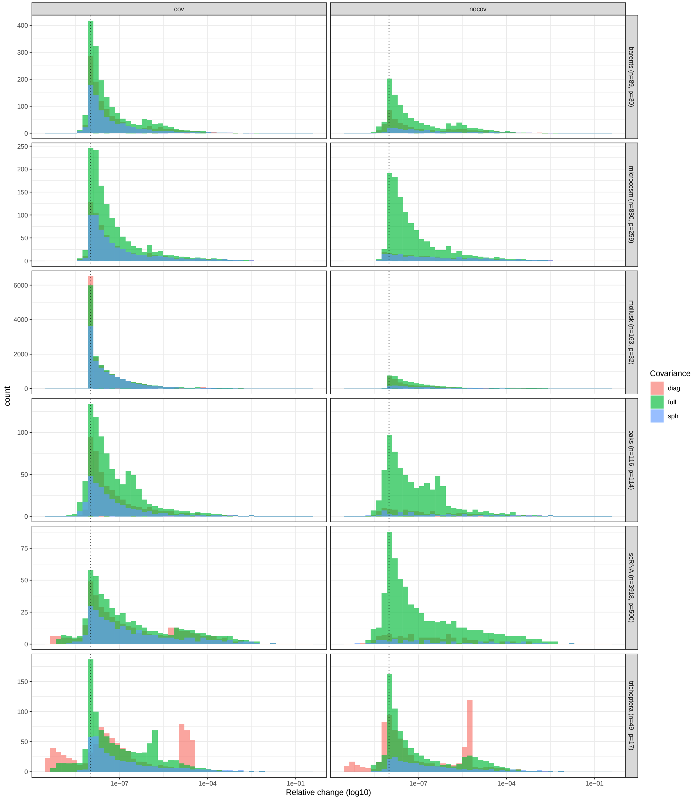
Distribution of per-step relative changes
