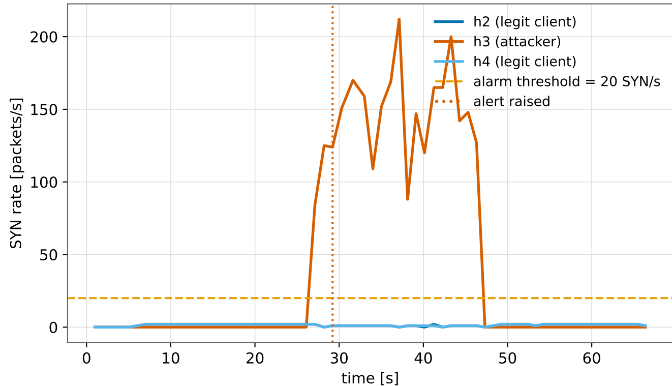
SYN flood detection: attacker traffic crosses the alarm threshold
