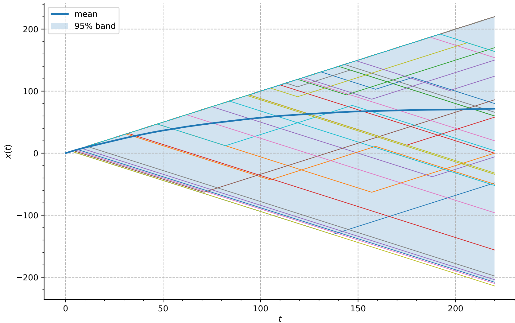
Fig. 1 Trajectory ensembles at b = 0
