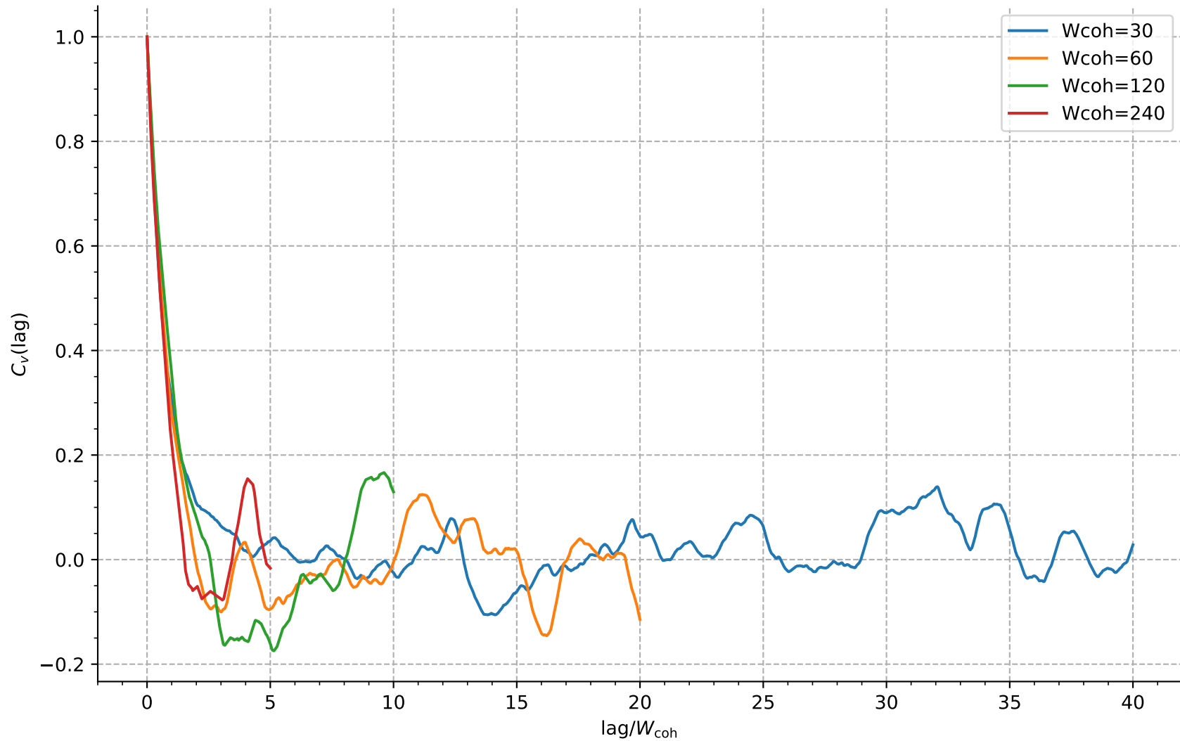
Fig. 4 Velocity autocorrelation collapse
