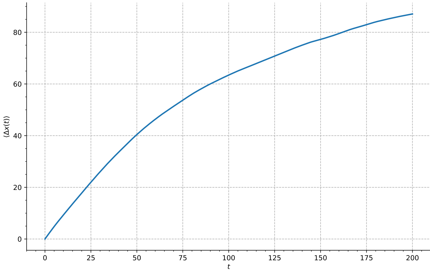
Fig. 2 Mean displacement \langle \Delta x(t) \rangle at b = 0
